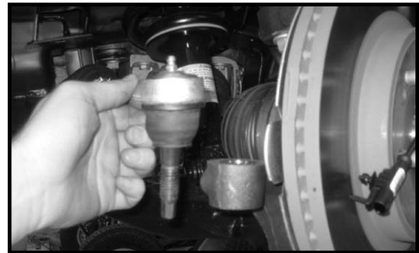
16. Working on the driver side, remove the lower hardware securing the strut to the lower control arm. The hardware may be discarded. Repeat procedure on the passenger side.
