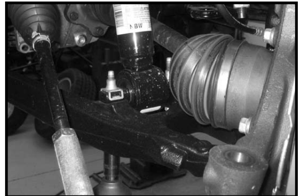
17. Working on the driver side, remove the upper clips off the upper strut studs. Remove the nuts holding the strut into the upper location and save. Remove the strut from the vehicle and remove and discard the lower attaching clips. Set the strut aside. Repeat procedure on the passenger side.
