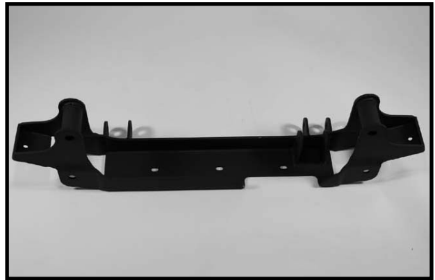
16955-17 (1) Rear cross member
